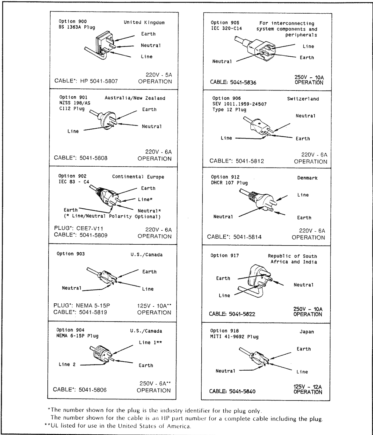
Figure 4-2. Power Cables
