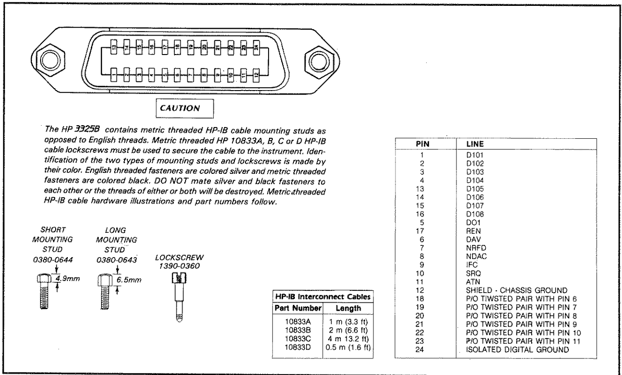
Figure 4-5. HP-IB Connector Information
