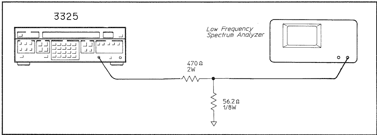
Figure 4-6. Harmonic Distortion Verification (High Voltage Output).
