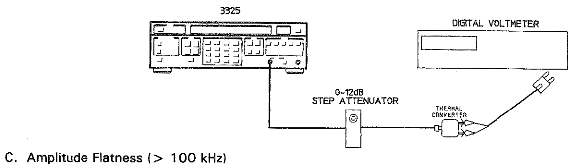
Figure 4-14. Amplitude Accuracy and Flatness.
