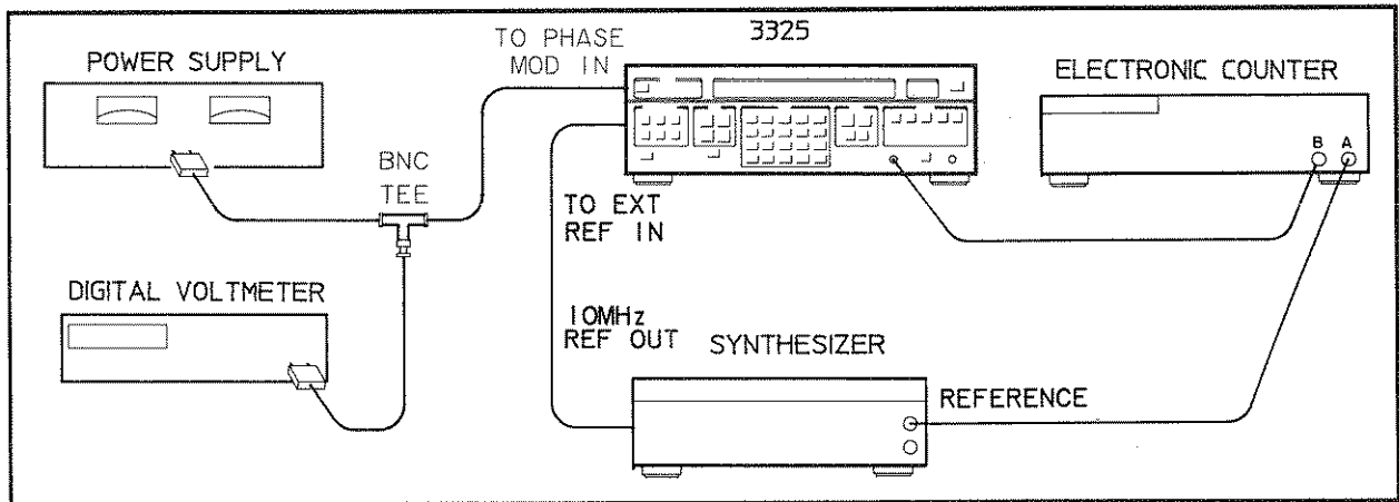
Figure 4-13. Phase Modulation Linearity.
